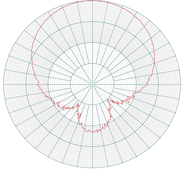
865 MHz
