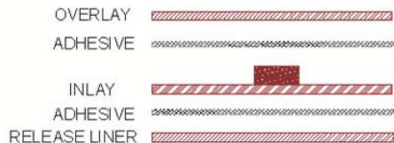
ALN-9862-WRW (White Wet Inlay)
