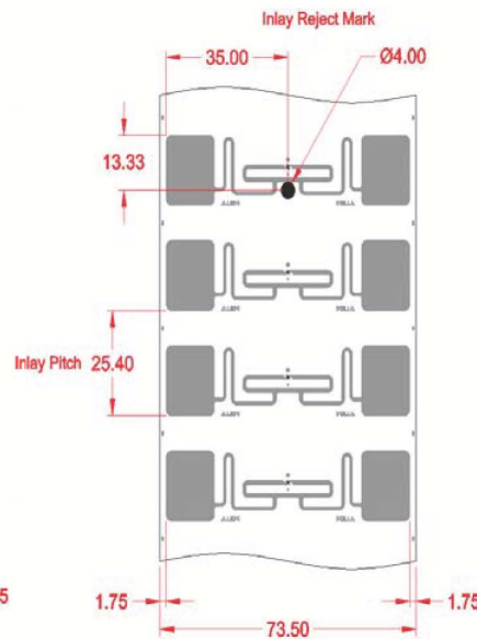
ALN-9862-SR (Dry Slit Roll)
