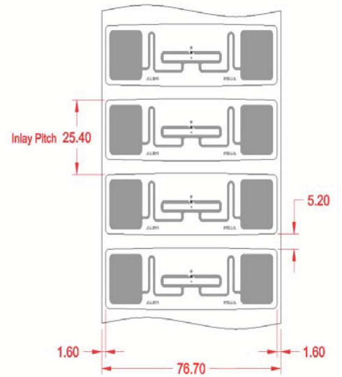
ALN-9862-WRW / WRC (White / Clear Wet Inlay)
