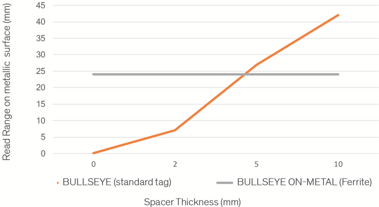
Comparison standard inlays with spacer and inlays with ferrite material
