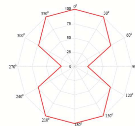
Read range (%) at various angle
