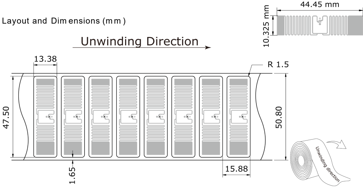
Construction (Reference thickness: mm)
