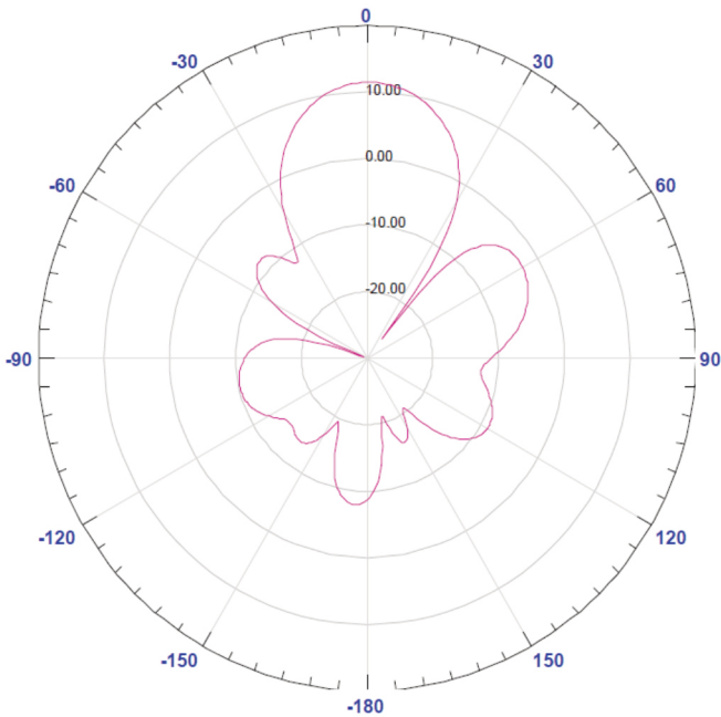
Antenna pattern (two-dimensional pattern)
