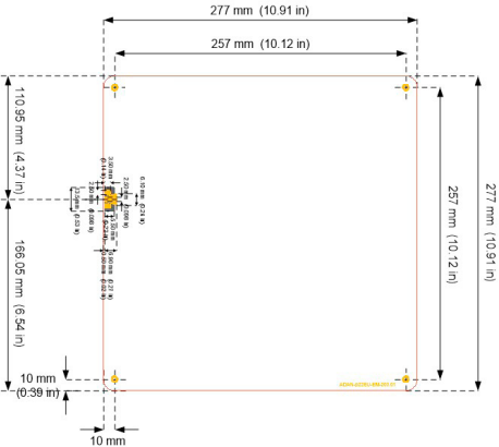
With edge mount connector
