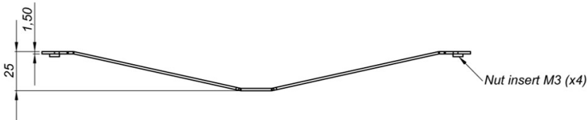
Mechanical Specifications (in Millimeters)
