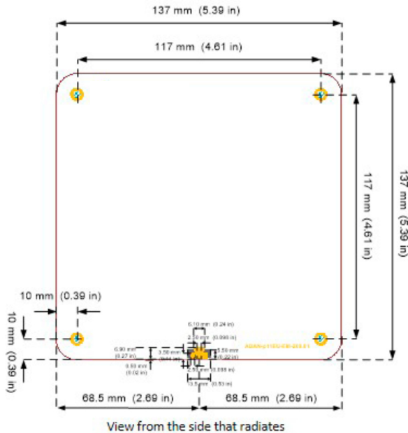
With edge mount connector
